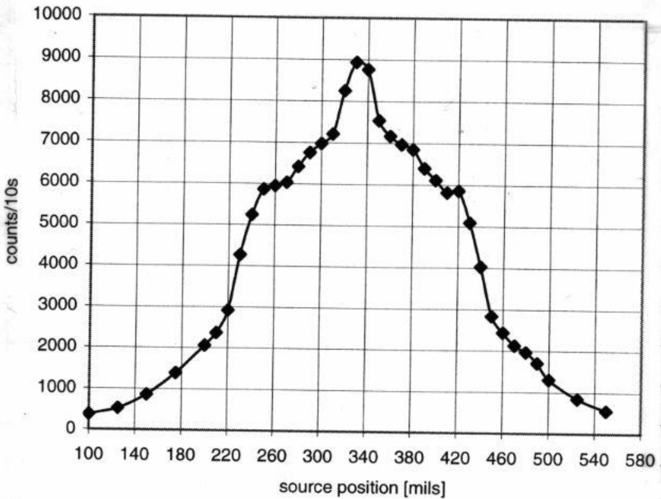
CKM prototype wire 7 scanned with Co57
